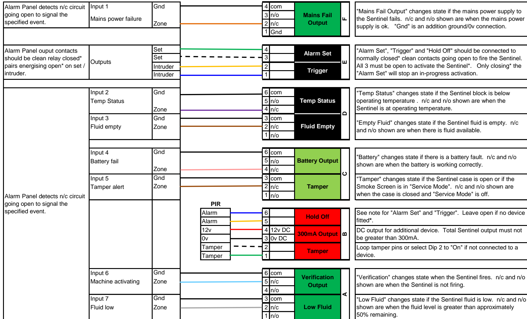
Alarm Panel or similar control device
